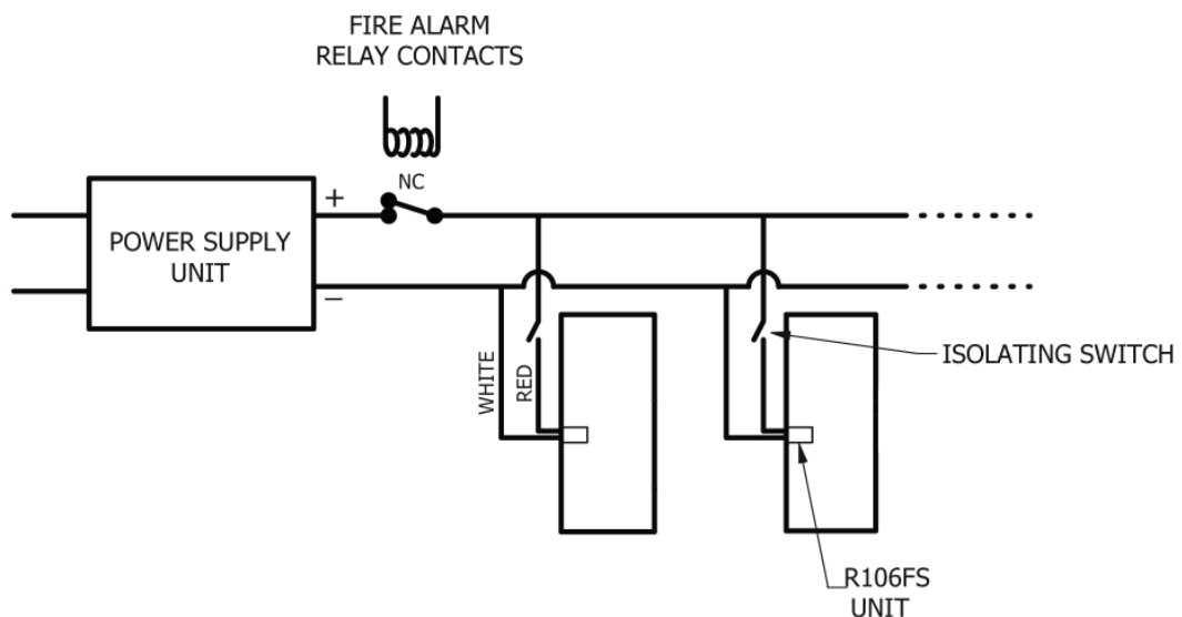
TYPICAL WIRING DIAGRAM
